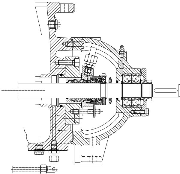
UEA with XEY, Cartex (PN25) double mechanicals seal
