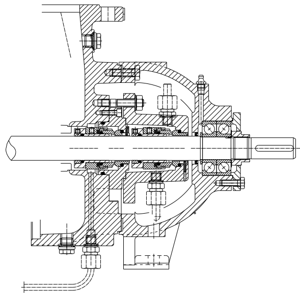
UEA with RBG, (PN40) double mechanicals seal
