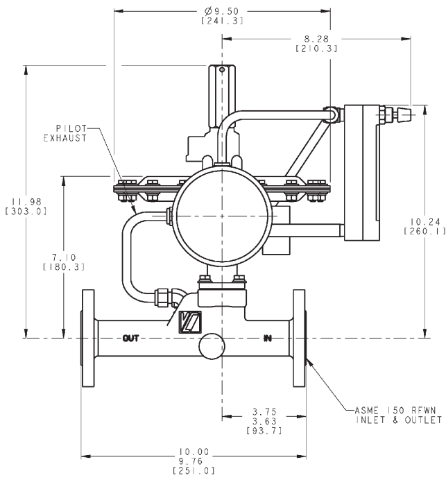
Integral 150# RF Flange Body with Gauges and Purge Meter
