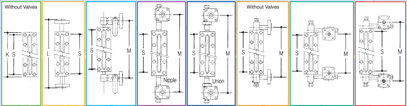
End Connected
